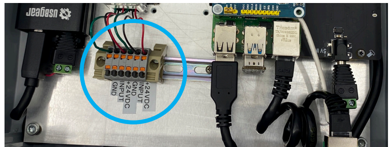
Base photo of Gateway. Some units include extra terminals.
